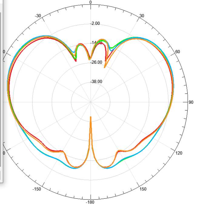
Gain Plot 5
